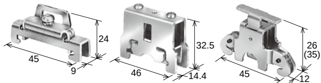
BNL6 (M4 Screw) (Tightening torque: 1.1 N·m) BNL8 (M4 Screw) BAL2 (Weight: Approx. 25.2g)
