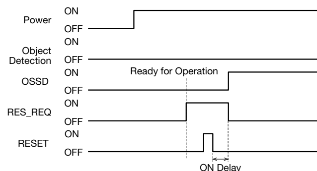
Time chart (manual start)
