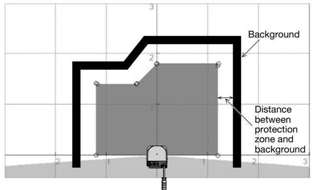
Auto configuration of protection zone
