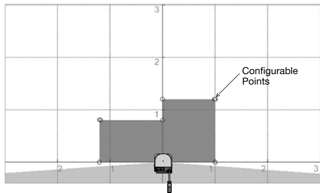
Auto configuration of protection zone
