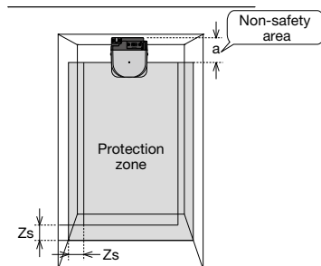
Safety distance (side view)
