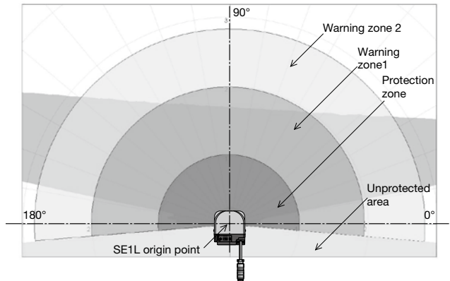
Manual configuration of protection zone
