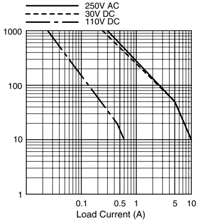
RU2 (Resistive Load)
